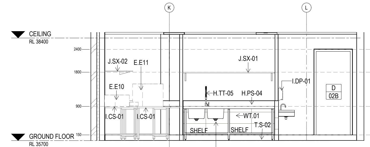
H ELEVATION CANTEEN/KITCHEN Scale: 1: 50
