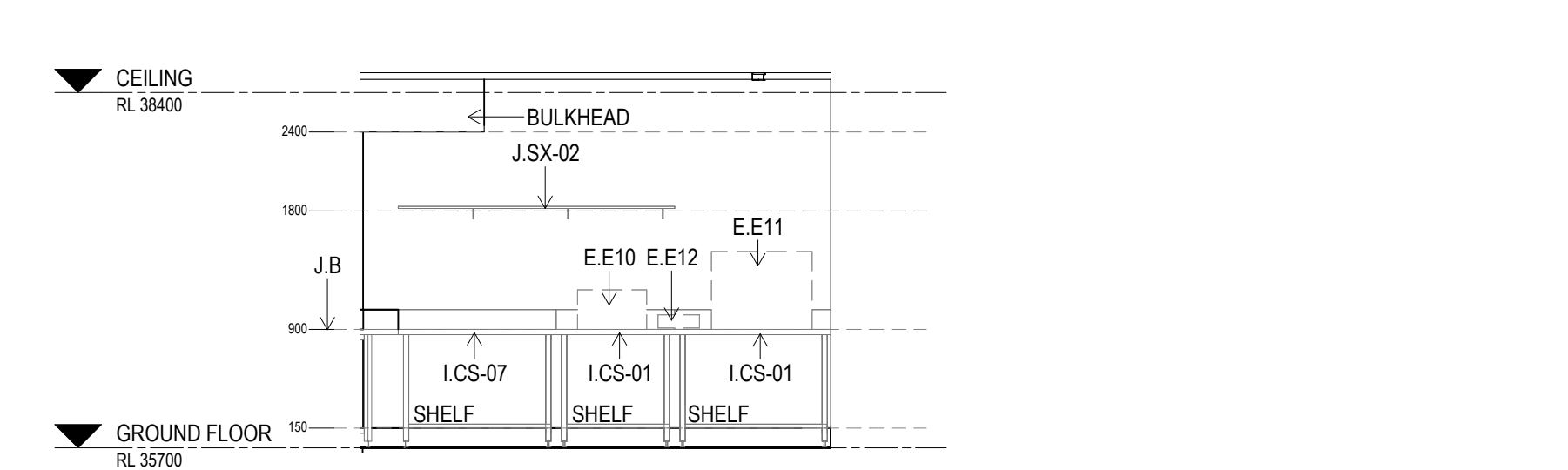
F ELEVATION CANTEEN/KITCHEN Scale: 1: 50
