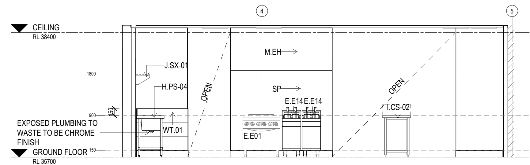
C ELEVATION CANTEEN/KITCHEN Scale: 1: 50
