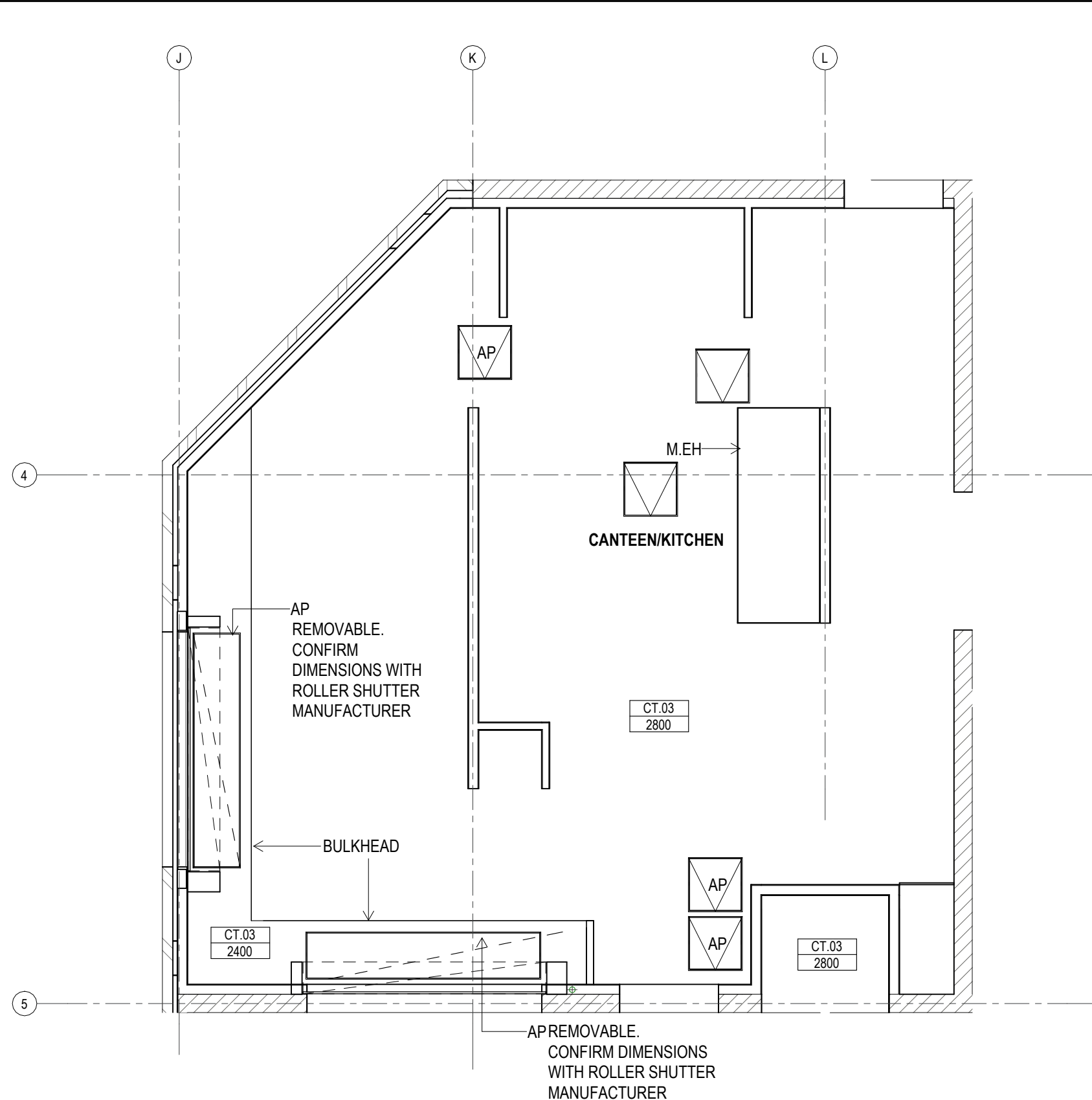
2 REFLECTED CEILING PLAN CANTEEN / KITCHEN Scale: 1: 50
