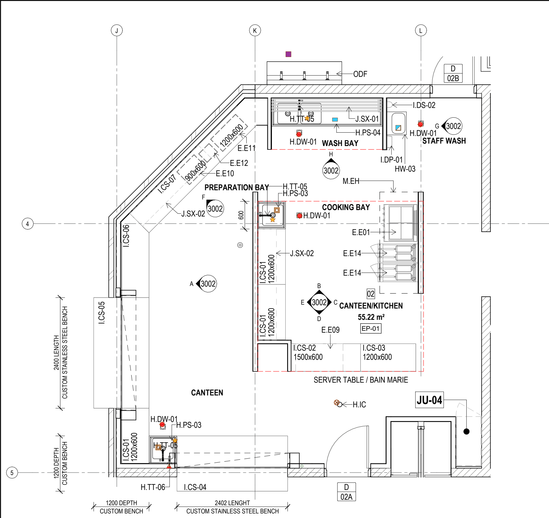
1 PLAN CANTEEN / KITCHEN Scale: 1: 50
