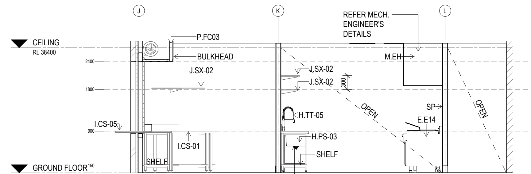
B ELEVATION CANTEEN/KITCHEN Scale: 1: 50
